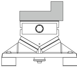
image: MD+UMS-ASF with substructure-rails, free-standing
